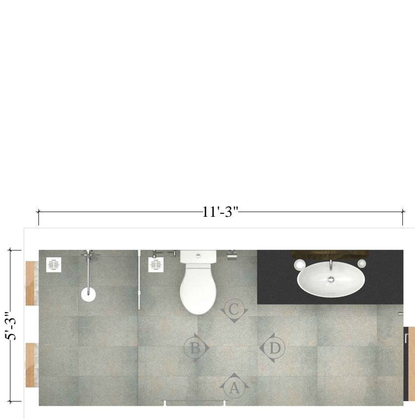
PLAN VIEW
