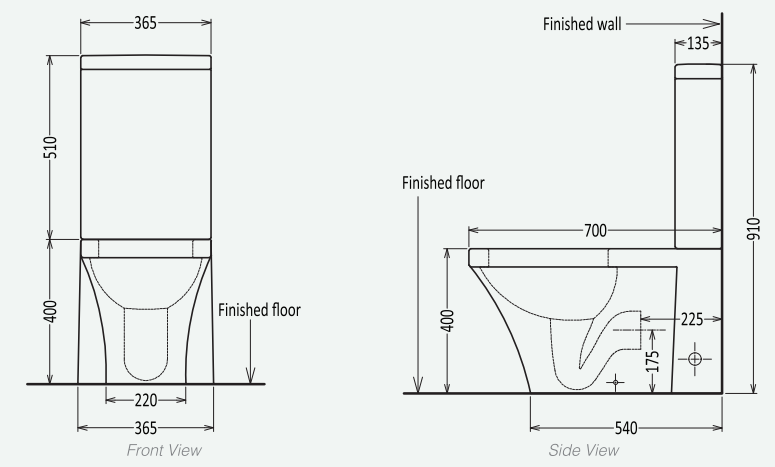
FLOOR-STANDING WATER CLOSET
